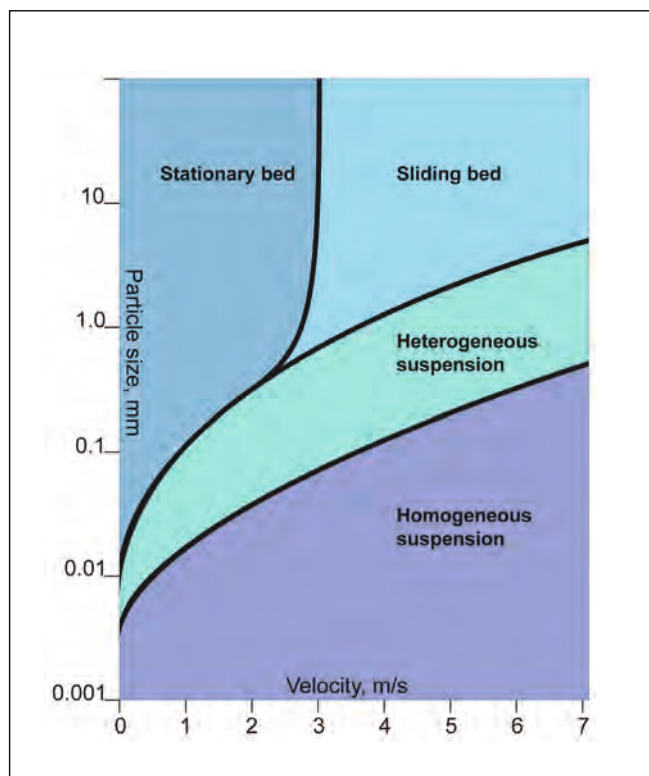
Example of flow configurations (sand density = 2700 kg/m 3 , pipe diameter 160 mm).
