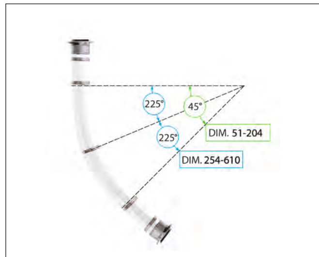
UNDERNEATH - Recommended number of clamps, support beams placed underneath the hose bend.
