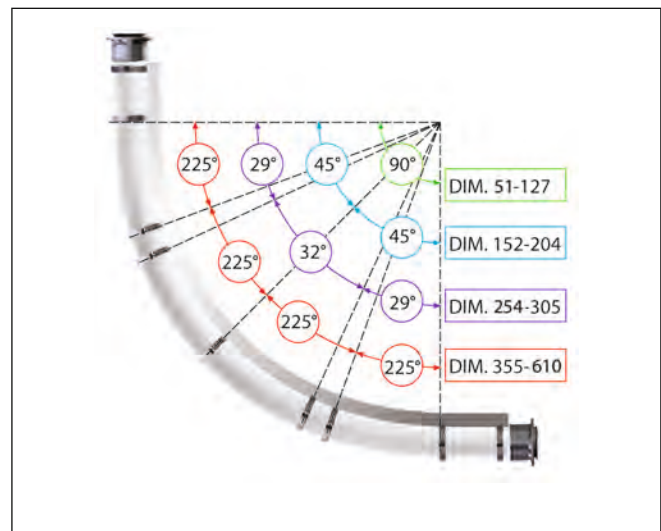
INSIDE - Recommended number of clamps, support beams placed on the inside of the hose bend.
